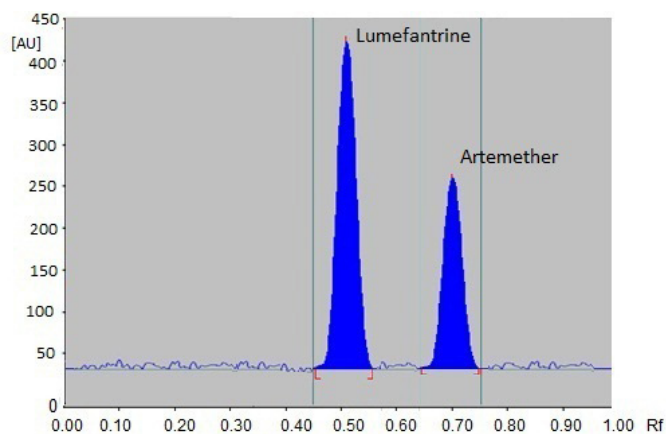
Figure 2: Chromatogram of standard ART (20 ng spot -1 ), Peak 1: R_f : 0.70 \pm 0.02 and LUM (100 ng spot -1 ), Peak 2: R_f : 0.52 \pm 0.02 , mobile phase- 2:6.5:0.5 v/v/v.
