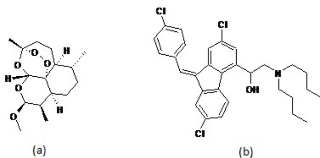
Figure 1: Structure of (a) artemether and (b) lumefantrine.
