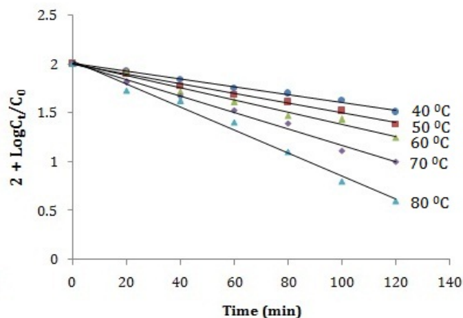
Figure 10: Pseudo first-order plots for the degradation of LUM with conc. HCl at various temperatures; C_t = Concentration at time t ; C_0 = Concentration at time zero.
