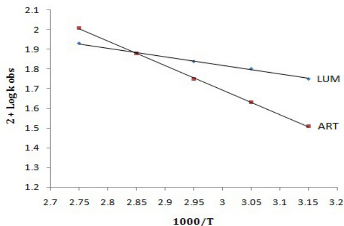
Figure 11: Arrhenius plot for the degradation of ART and LUM in presence of Conc. HCl.
