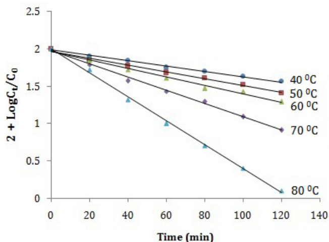
Figure 9: Pseudo first-order plots for the degradation of ART with conc. HCl at various temperatures; C_t = Concentration at time t ; C_0 = Concentration at time zero.
